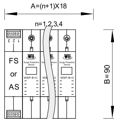
Modular Surge Protection Devices With Monitors
