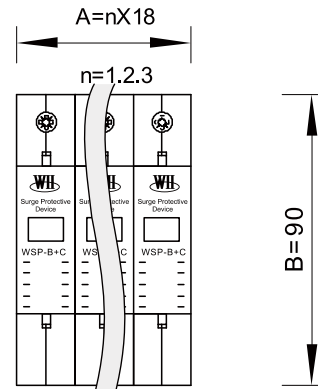
Modular Surge Protection Devices
